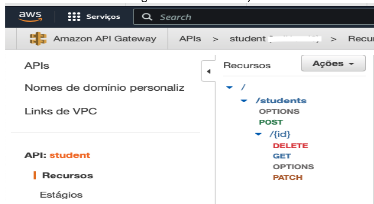
Figura 6 - API Gateway
